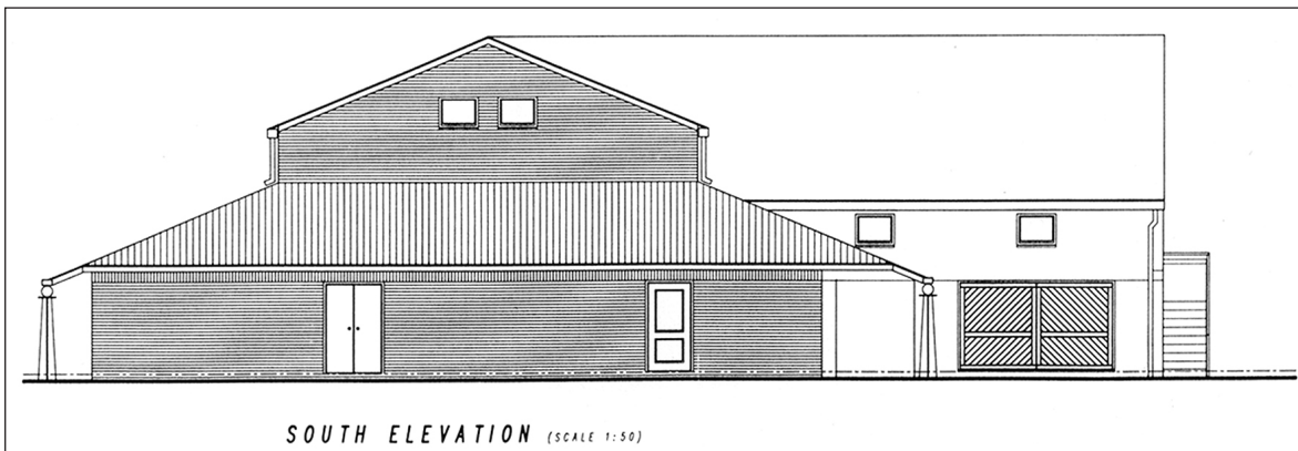
South and west elevations of the new wraparound extension
